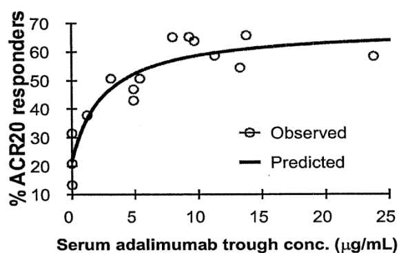
Figure 1: Concentration-Efficacy Relationship
